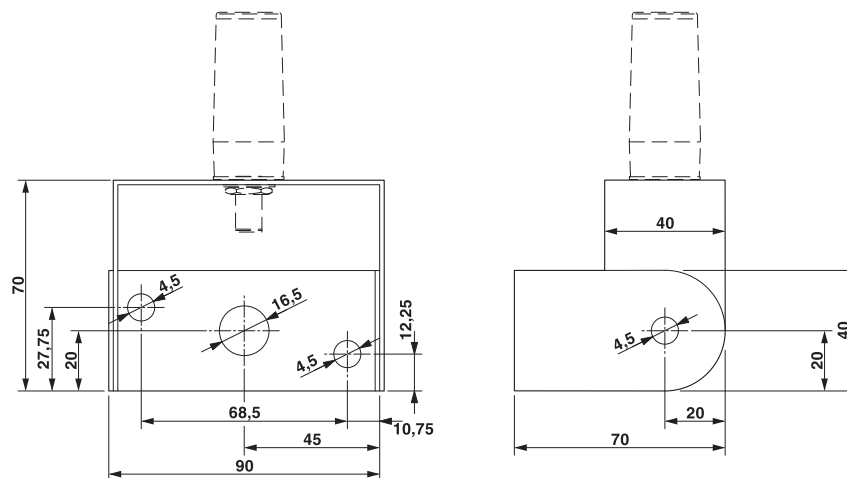
Dimensional drawing
