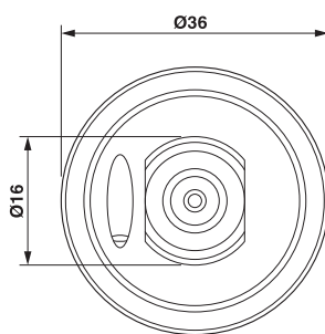
Dimensional drawing
